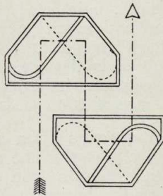
Porro-prisms broad shape
