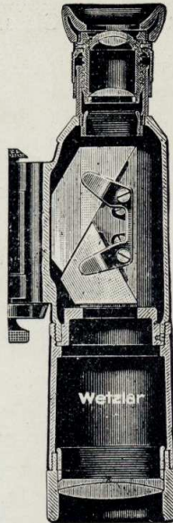
Hensoldt Patent Dialyt-prisms
